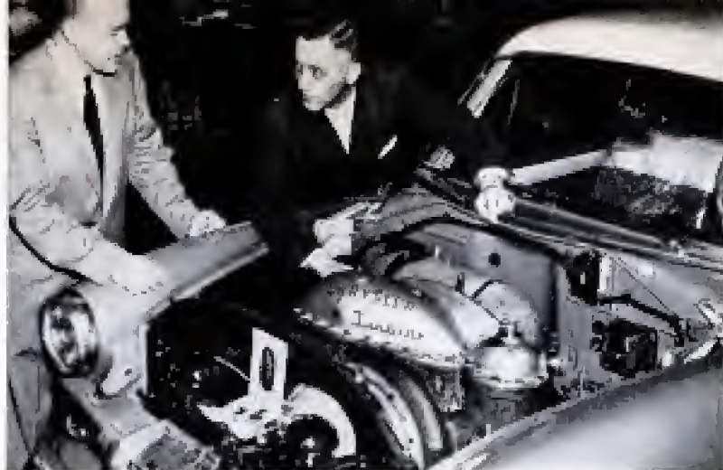
Fitting neatly under the hood of a Plymouth, the turbine is simple, has a fifth as many parts as a piston engine
